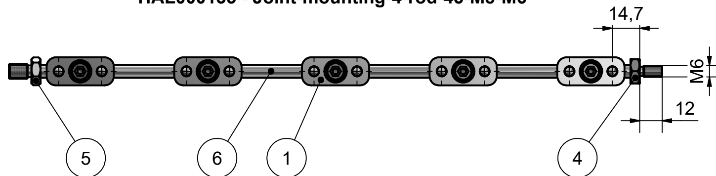
HAL000133 - Joint-mounting-4-rod-45-M8-M6
