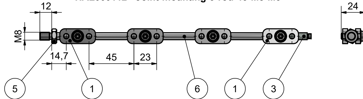
HAL000112 - Joint-mounting-3-rod-45-M8-M5
