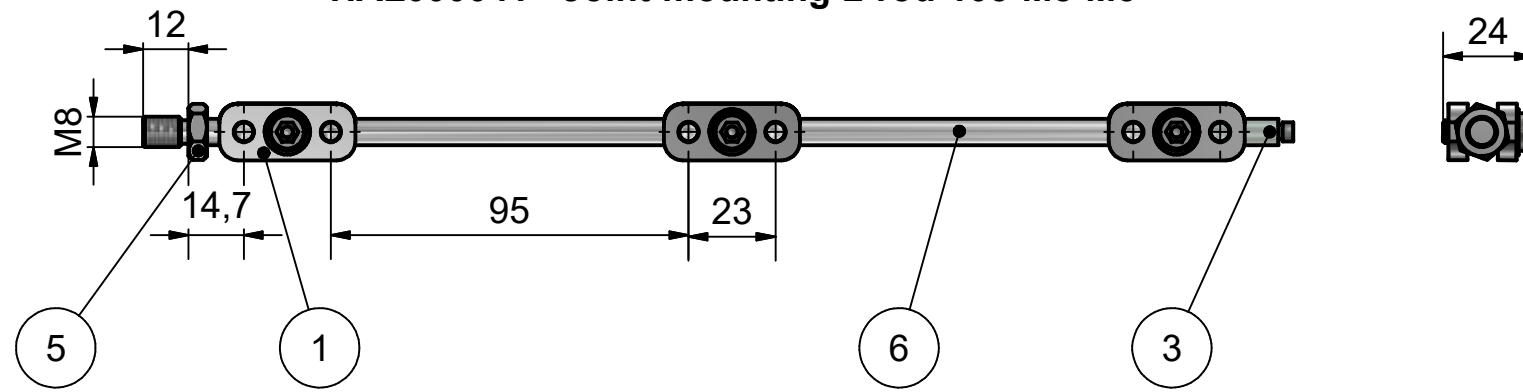
HAL000041 - Joint-mounting-2-rod-105-M8-M5
